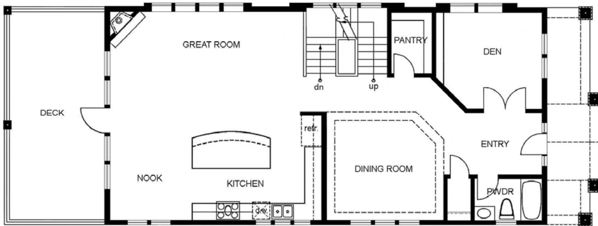
MAIN FLOOR
