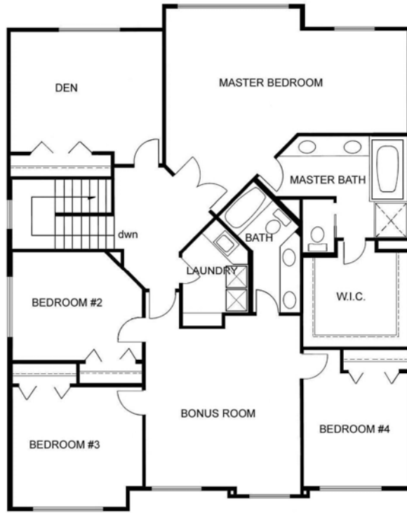
UPPER FLOOR
